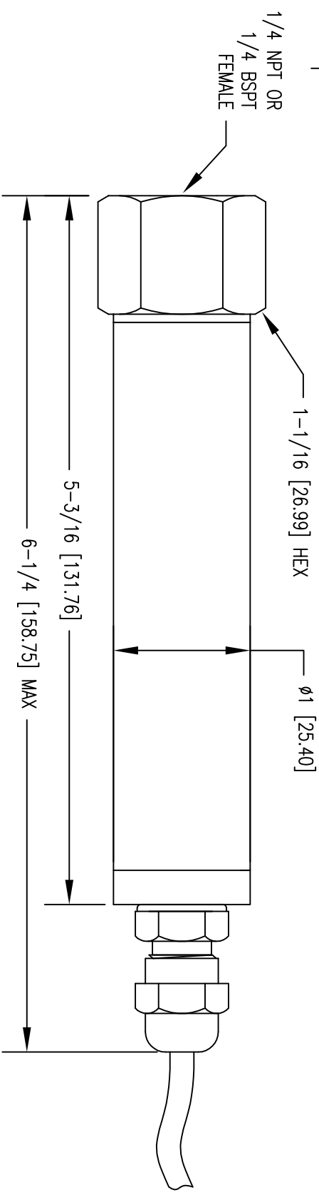
FEMALE NPT/BSPT CONNECTOR WITH CABLE GLAND
