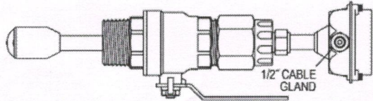
Hot-Tap Option
